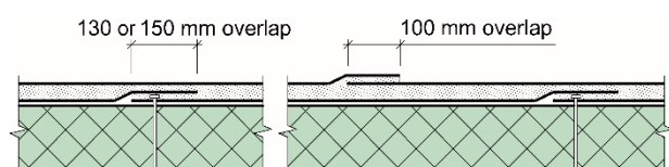
Fig. 2. Fastening and overlap of Derbigum Totaltekkings
